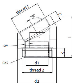
Outlet directions: 45° elbow / MAVI-Mxx/01
