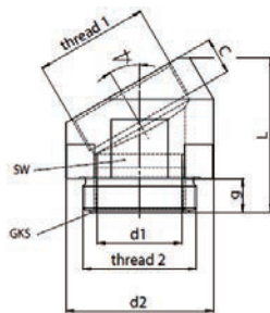
Outlet directions: 45° elbow / MAVI-Pxx/01
