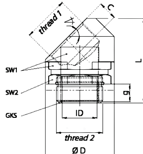
Outlet directions: 45° elbow / MAVIK-Mxx/01
